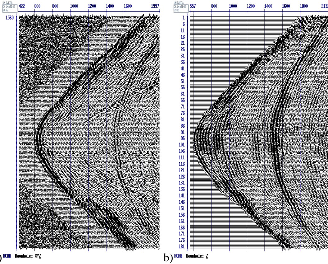
Fig. 3. 3D VSP data: a) – a raw common receiver gather; b) – reflected P-waves after selection.
