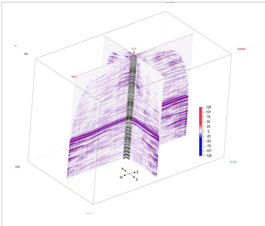
Fig. 2. Seismic images obtained from walkaway data in comparison with VSP primary reflection trace.
