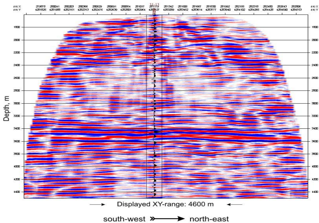
Fig. 4. A seismic image obtained from 3D VSP data in comparison with VSP primary reflection trace.
