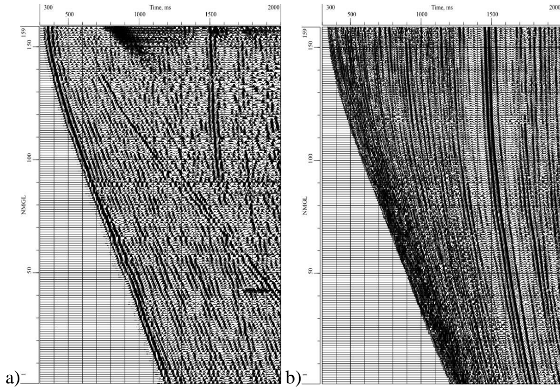
Fig. 1. Walkaway data: a) – a raw common receiver gather; b) – reflected P-waves after selection, spike deconvolution, and stacking of all levels.
