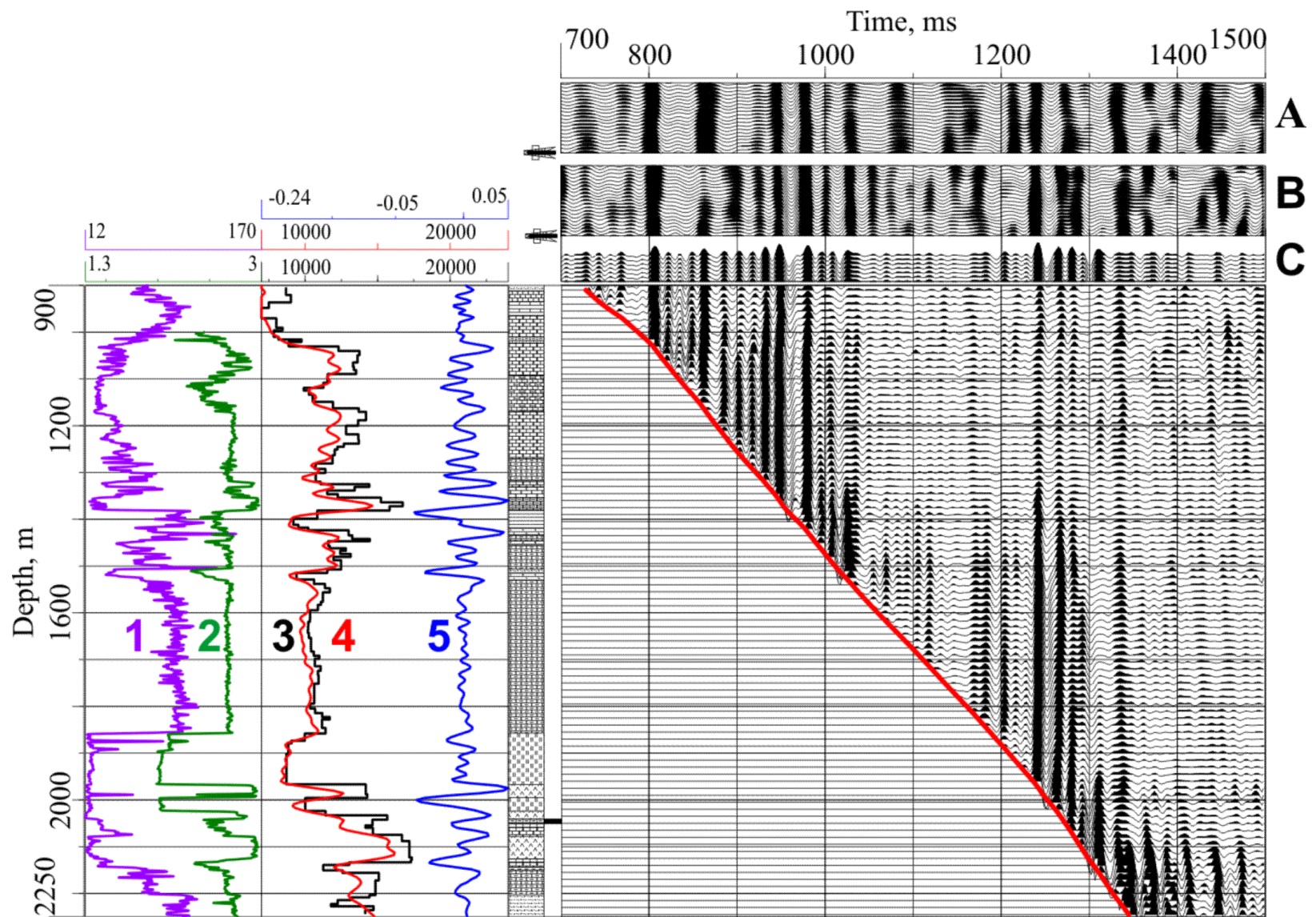
Fig. 4. VSP field tie to log data and surface seismics: 1 – acoustic log, 2 – gamma ray log, 3 – acoustic impedance derived from log data, 4 – acoustic impedance derived from VSP data, 5 – primary reflection trace (in depth scale); A – a CDP section fragment, B – the same CDP section fragment after deconvolution by VSP trace, C – primary reflection trace (in time scale).
