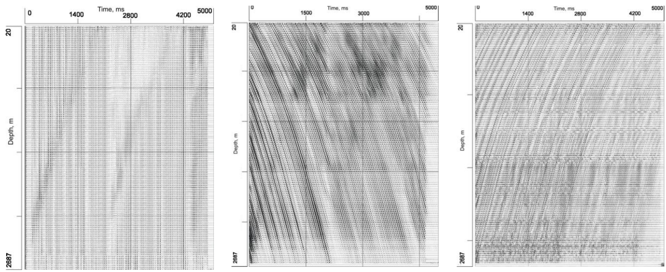
Fig.3. Autocorrelation wave-fields after selection procedure
