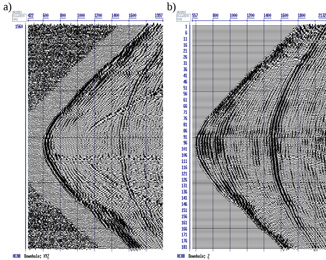
Fig. 3. 3D VSP data: a) – a raw common receiver gather; b) – reflected P-waves after selection.
